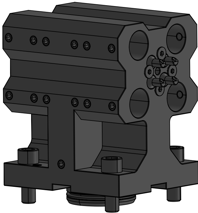
90 DEGREE STATIC TOOL OUTPUT: 1" BORING BAR MAIN & SUB QUAD COOLANT: EXTERNAL
